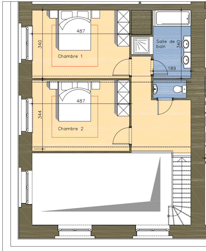
Mezzanine
